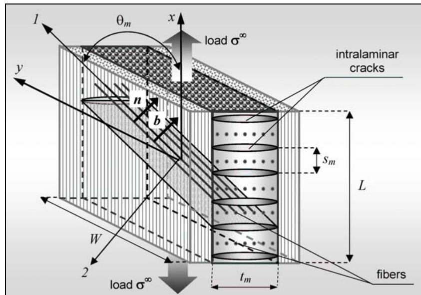
Figure 2. Orientation of intralaminar matrix cracks within off-axis ply
