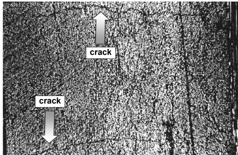
Figure 1. Transverse matrix cracking in [0, 90_8, 0] cross-ply laminate
