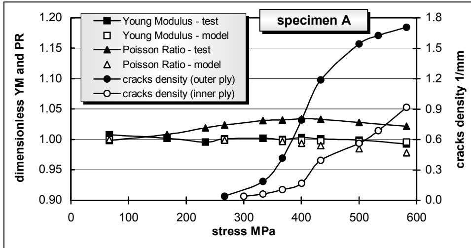
Figure 14. Dimensionless YM, PR and crack density vs. stress for set # 1 specimen A
