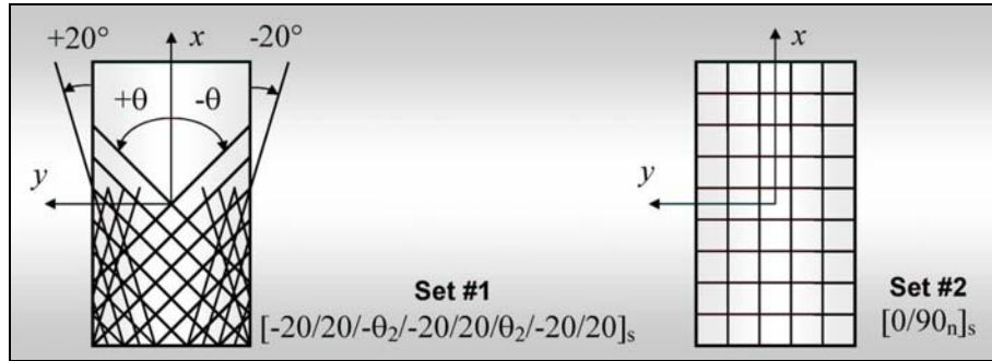
Figure 7. Two sets of test specimens
