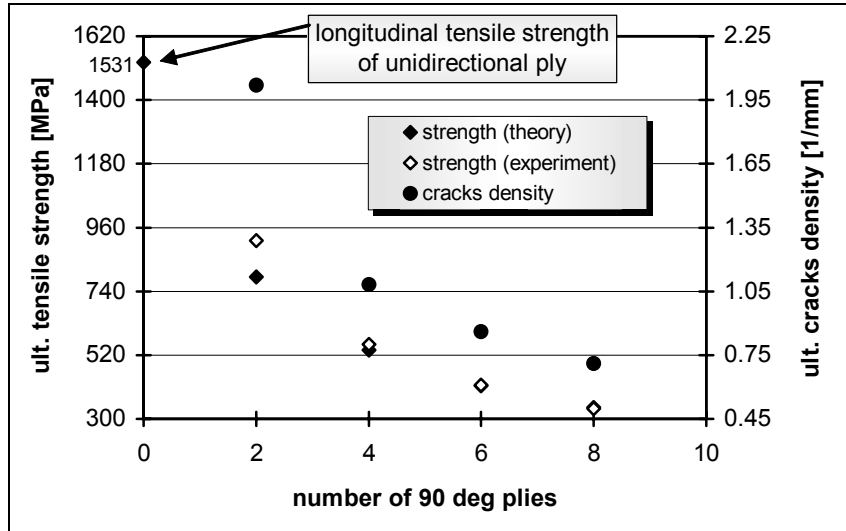
Figure 9. Ultimate tensile strength and crack density vs. number of 90° plies
