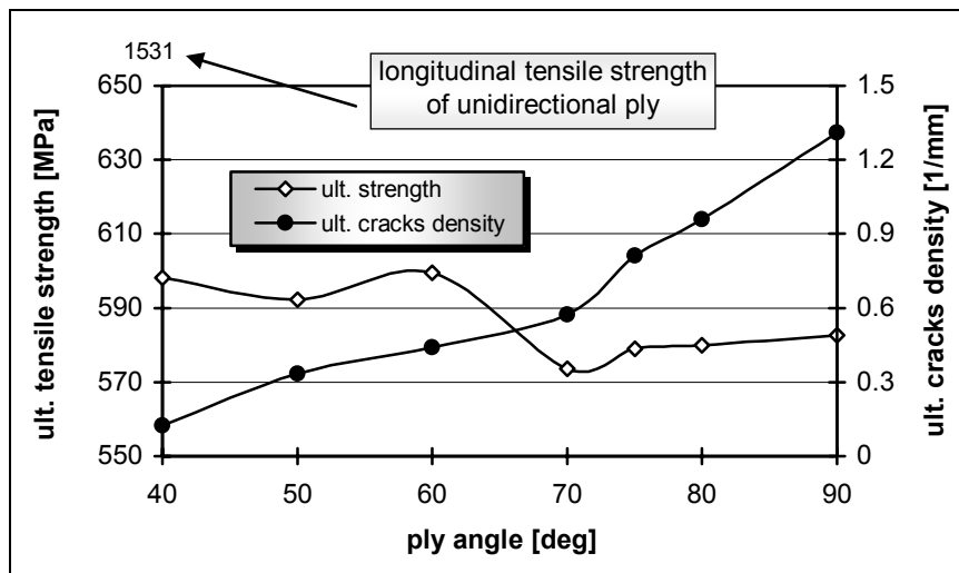
Figure 10. Ultimate tensile strength and crack density vs. damaging ply angle
