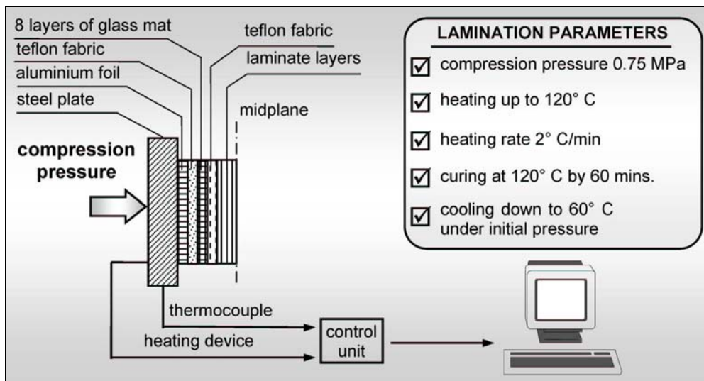
Figure 6. Lamination of the specimen material
