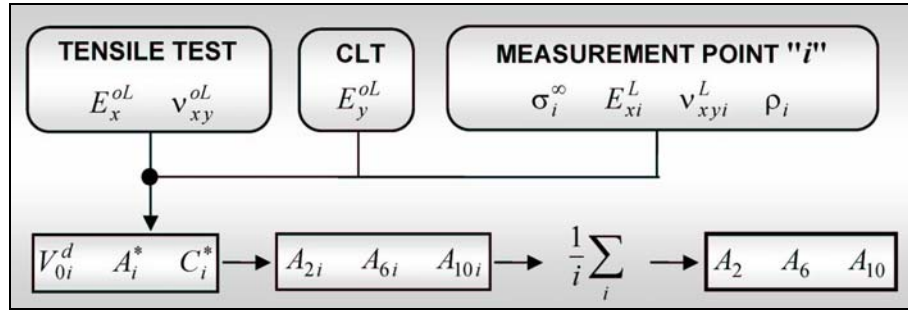
Figure 4. The procedure of calculation of material parameters
