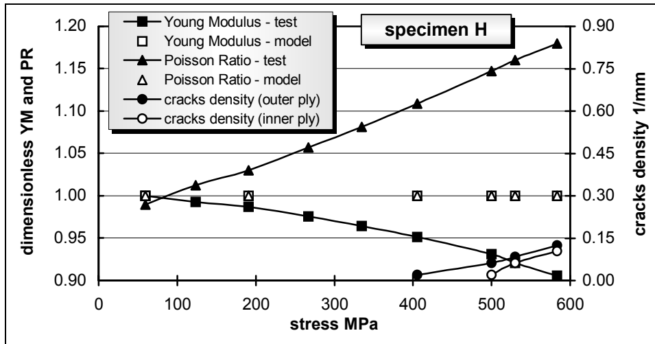
Figure 15. Dimensionless YM, PR and crack density vs. stress for set # 1 specimen H
