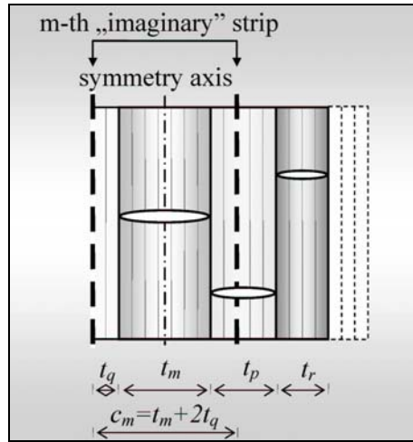
Figure 3. Construction of imaginary strip
