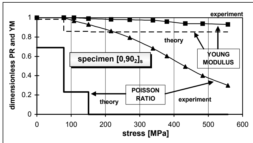
Figure 11. Dimensionless YM and PR - theoretical predictions and test data
