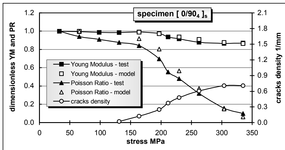
Figure 13. YM, PR and crack density as functions of applied load for [0/90_4]_s specimen
