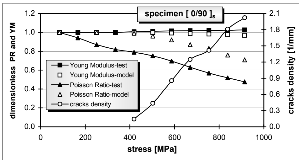
Figure 12. YM, PR and crack density as functions of applied load for [0/90]_s specimen
