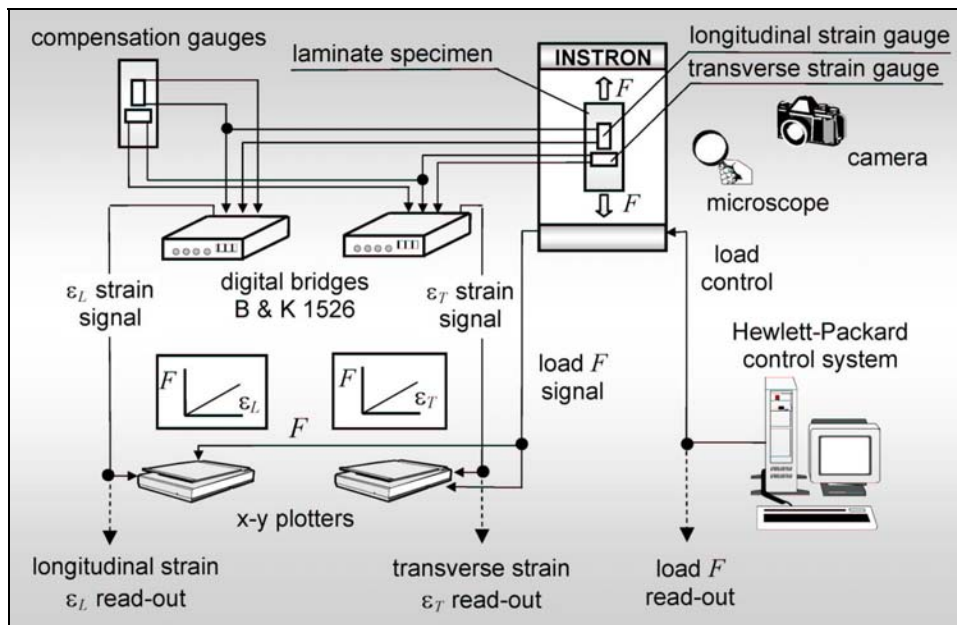
Figure 8. The scheme of testing instrumentation
